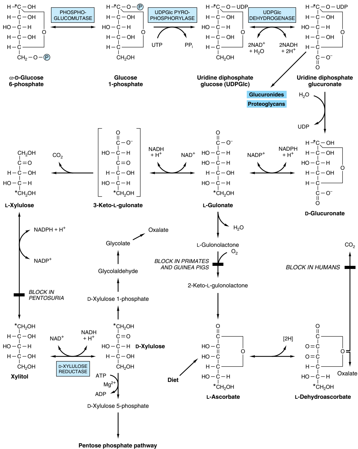
Figure 20-4. Uronic acid pathway. (Asterisk indicates the fate of carbon 1 of glucose; \text{P} , -\text{PO}_3^{2-} .)
