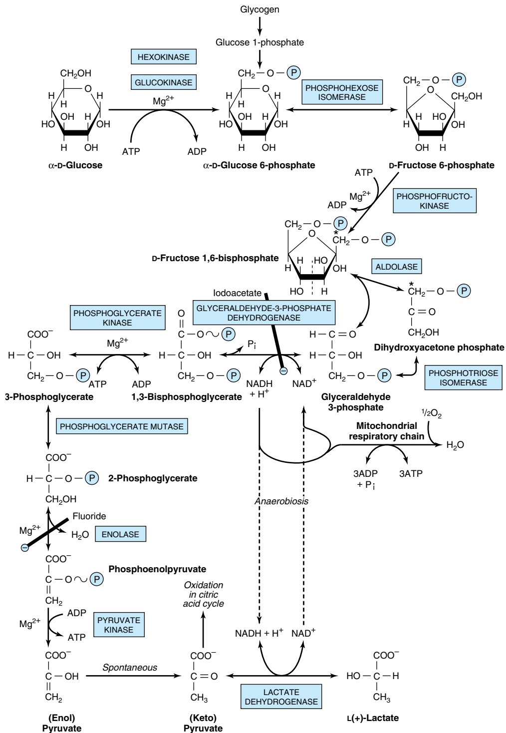
Figure 17-2. The pathway of glycolysis. (Ⓟ, — PO_3^{2-} ; P_i , HOPO_3^{2-} ; ⊖, inhibition.) At asterisk: Carbon atoms 1–3 of fructose bisphosphate form dihydroxyacetone phosphate, whereas carbons 4–6 form glyceraldehyde 3-phosphate. The term “bis-,” as in bisphosphate, indicates that the phosphate groups are separated, whereas diphosphate, as in adenosine diphosphate, indicates that they are joined.
