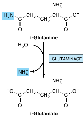
Figure 29–8. The glutaminase reaction proceeds essentially irreversibly in the direction of glutamate and \text{NH}_4^+ formation. Note that the amide nitrogen, not the \alpha -amino nitrogen, is removed.
